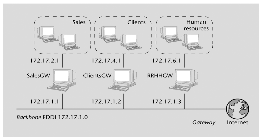
Figure 1. Configuration of segments and gateways in an intranet
